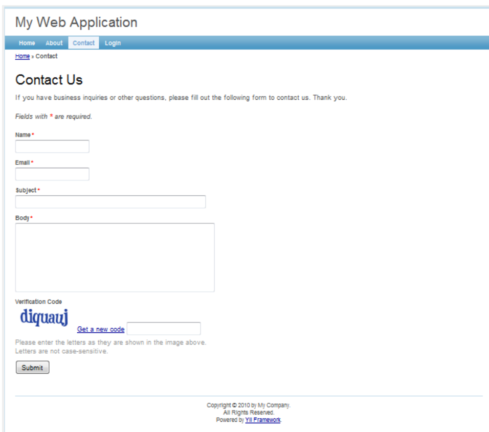
Figure 1.2: Contact page
