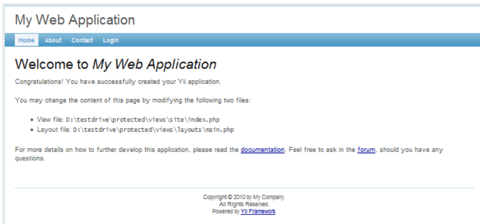
Figure 1.1: Home page
